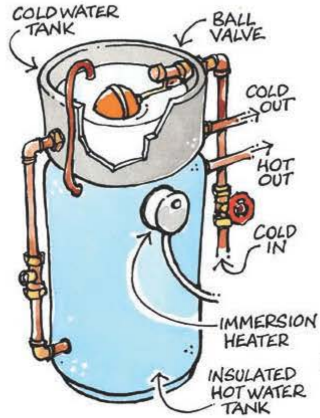
HOT WATER CYLINDER
