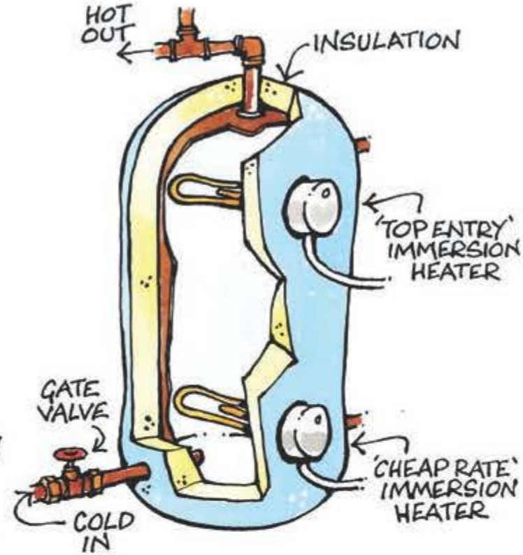
COMBINATION TANK
